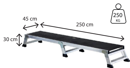
UPDOWNLP250: 50 cm x 45 cm x 30 cm
