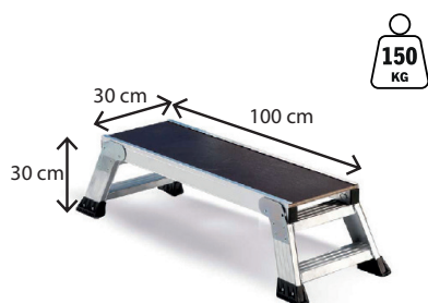
UPDOWNP100: 100 cm x 30 cm x 30 cm
