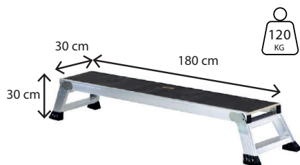
UPDOWNNP180: 80 cm x 30 cm x 30 cm
