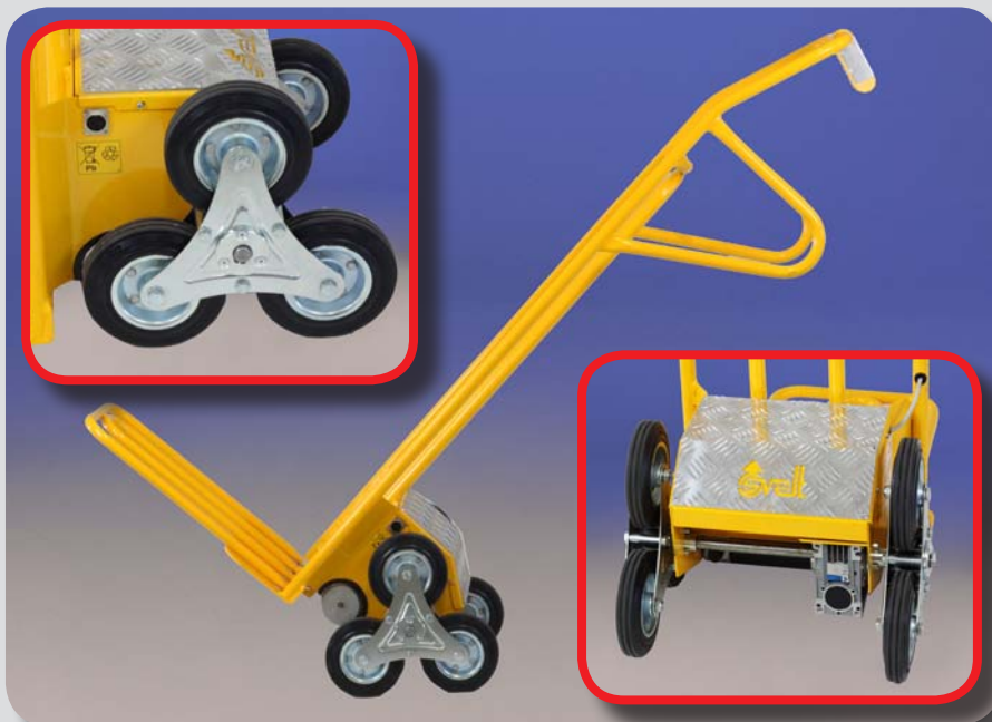
AUTOMATIC BATTERY CHARGER: Just plug in the charger and in 4 hours the handtruck is ready for use with the maximum charge.
